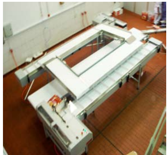
Layout with 2 Multipacks and circular conveyors
